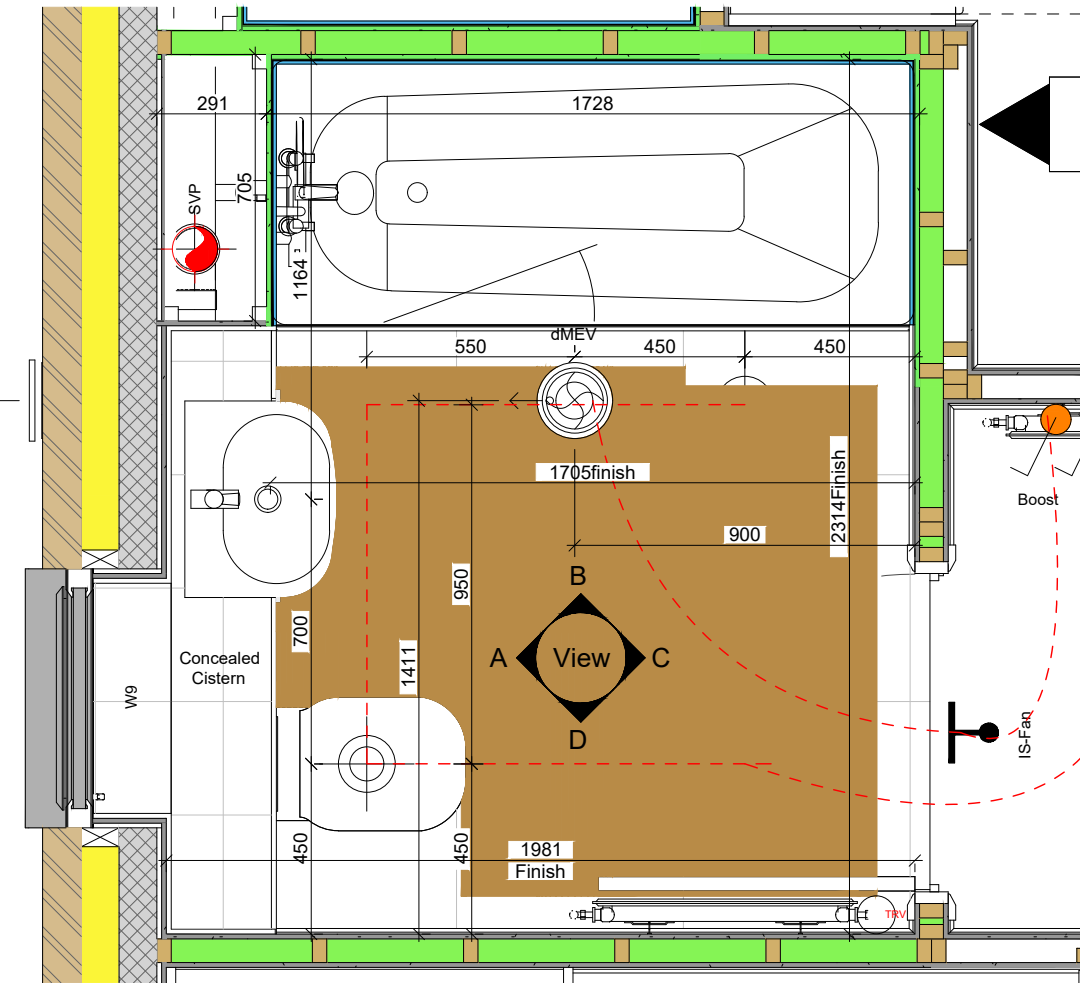
1 Bathroom Layout 1 : 20
