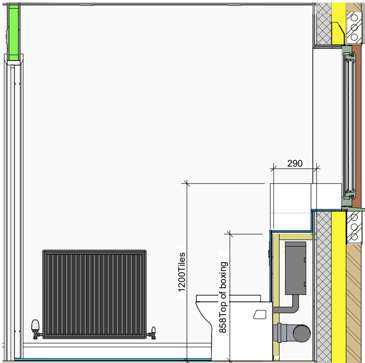
D Bathroom - View D 1 : 25 Plots 08, 14, 50 (AS) & 01, 03, 09, 18, 19, 49 OPP
