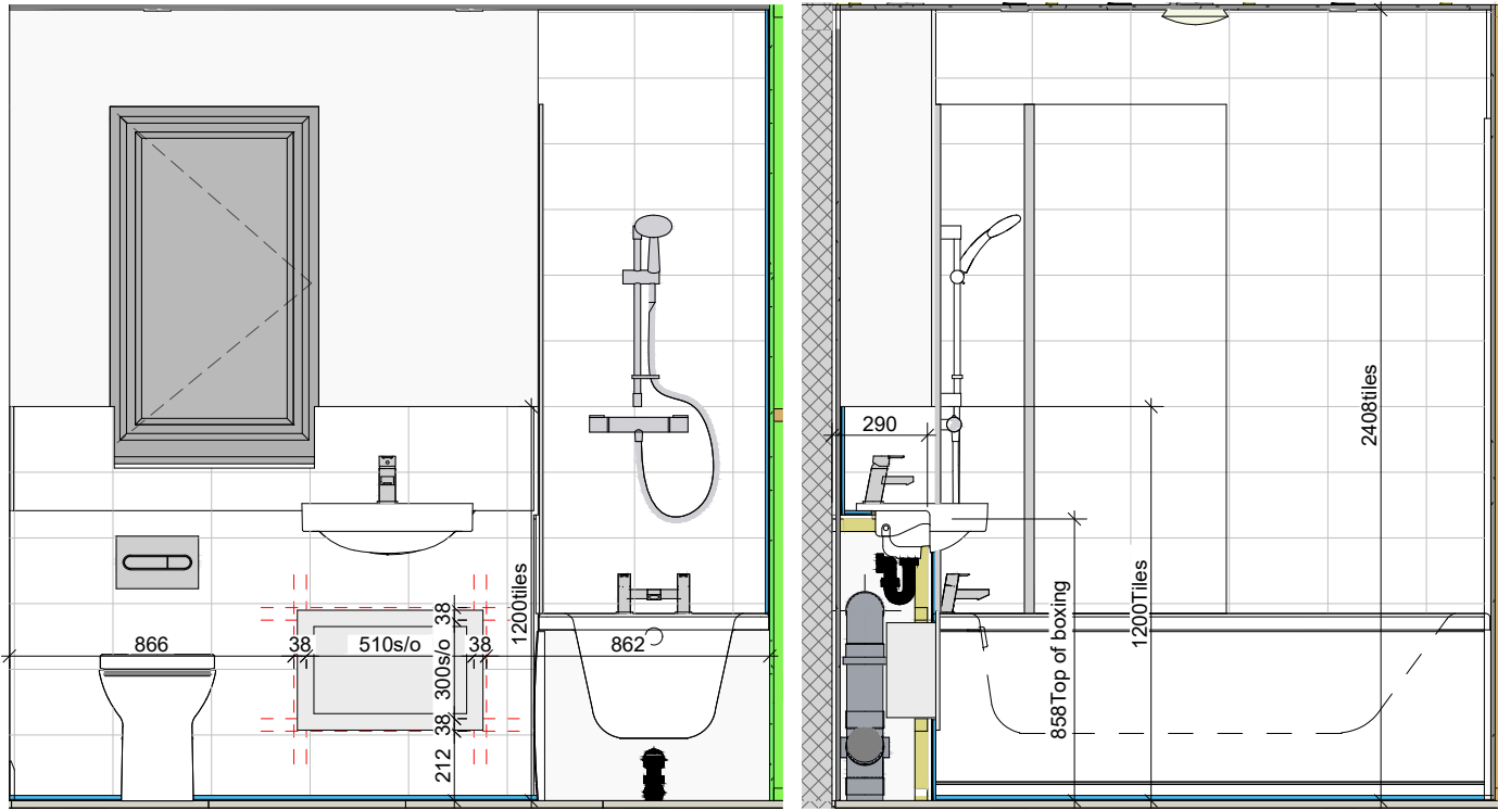
A Bathroom - View A 1 : 25
